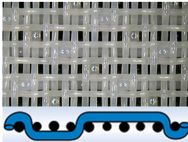
1.5-layer 5-shed with Extra Yarns
